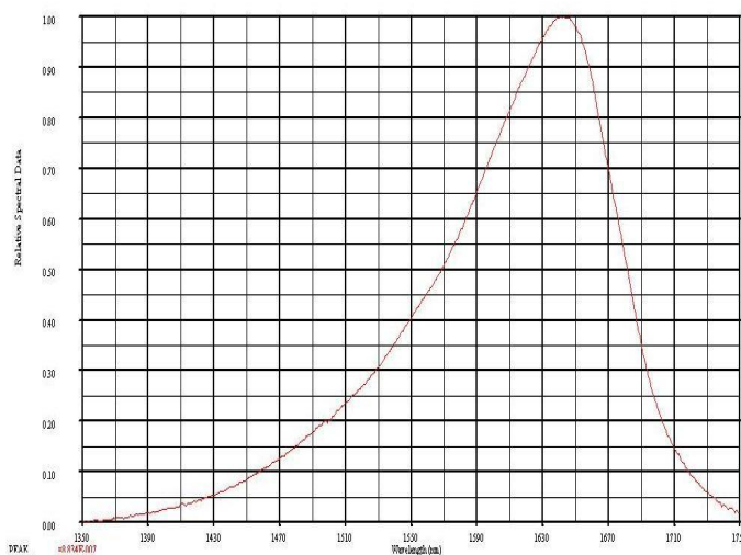
SPECTRAL OUTPUT
