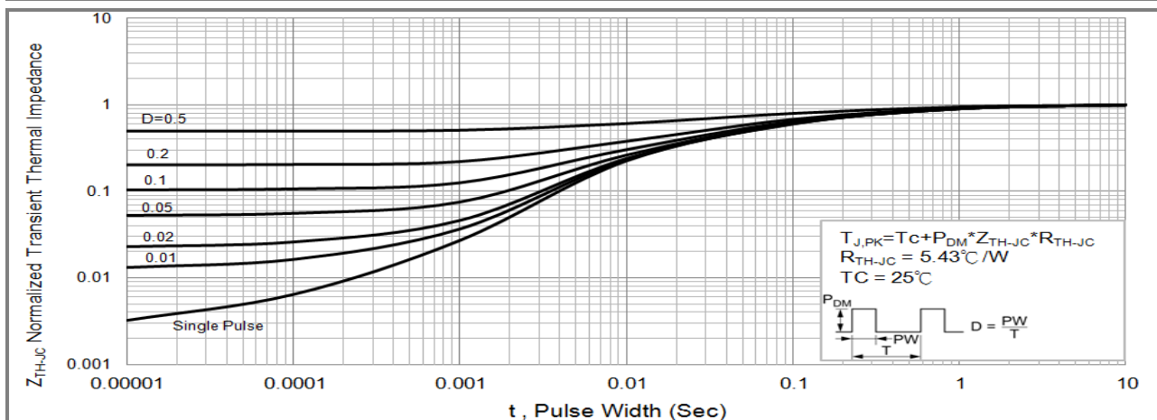
Fig.15 PJF Normalized Transient Thermal Impedance vs. Pulse Width
