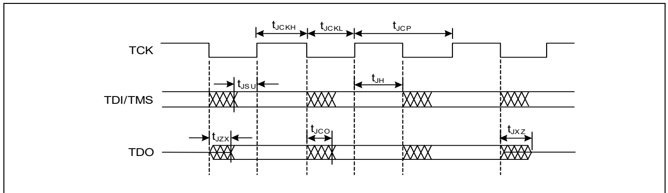
Figure 27-22 JTAG specifications
