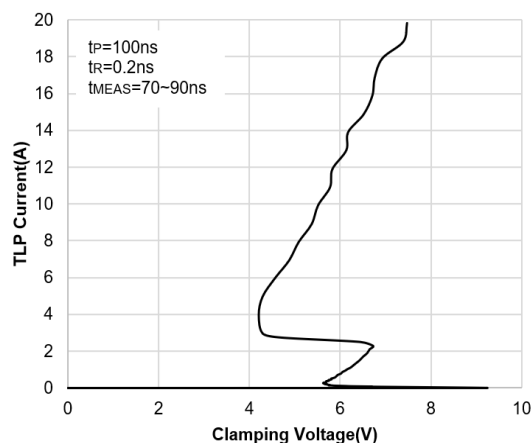
TLP I/V Curve
