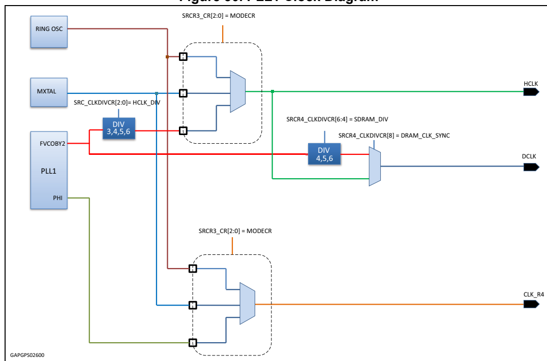
Figure 30. PLL1 Clock Diagram
