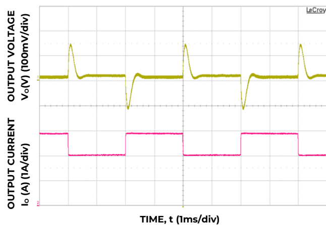
Figure 6. Dynamic Load Change Transient Response from 50% to 75% to 50% of Full Load at Room Temperature and 48V; 0.1A/\mu s , C_{o,ext} = 220\mu F .
