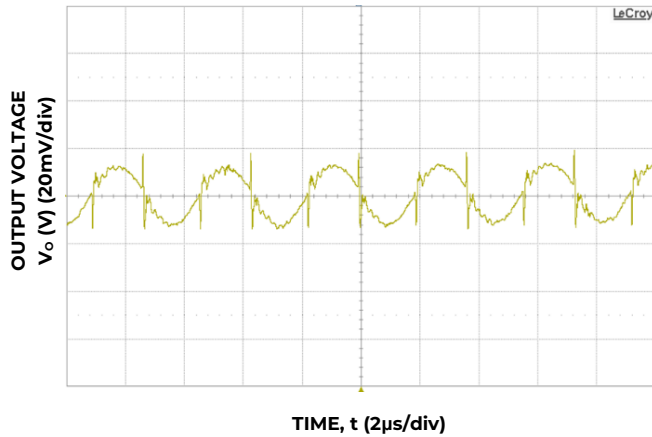
Figure 2. Typical Output Ripple and Noise at Room Temperature and 48V; I_o = I_{o,max} ; C_{o,ext} = 220\mu F .
