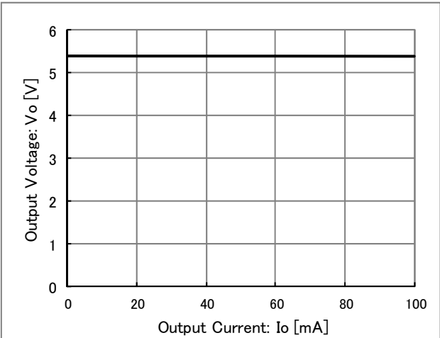
Figure 9. I_o - V_o
