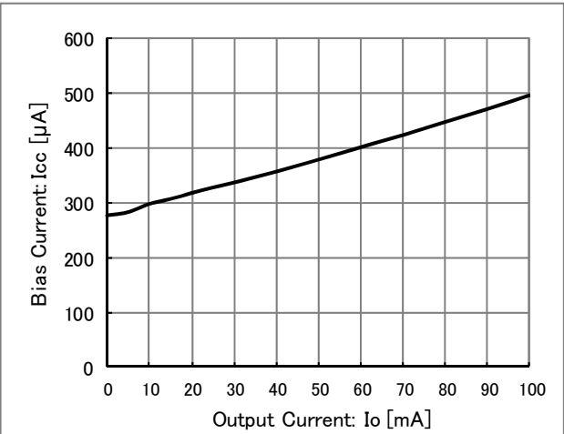
Figure 8. I_o - I_{cc}
