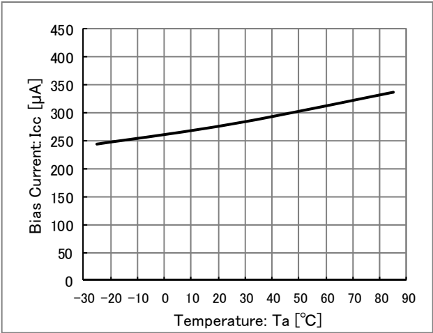
Figure 7. T_a - I_{cc}
