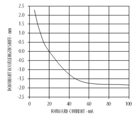
Figure 5 Dominant Wavelength Shift vs. Forward Current
