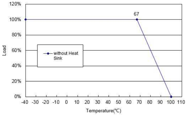
FM30-100 Typical Power De-rating Curve
