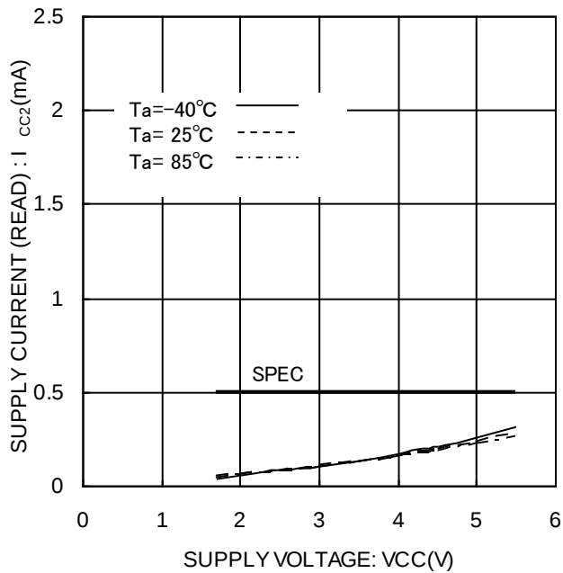
Figure 16 Supply current (READ) I_{CC2}(\text{READ}, f_{SK}=1\text{MHz}) .
