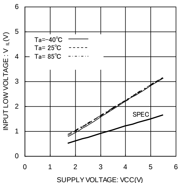
Figure 5. Input low voltage V_{IL}(\text{CS,SK,DI})
