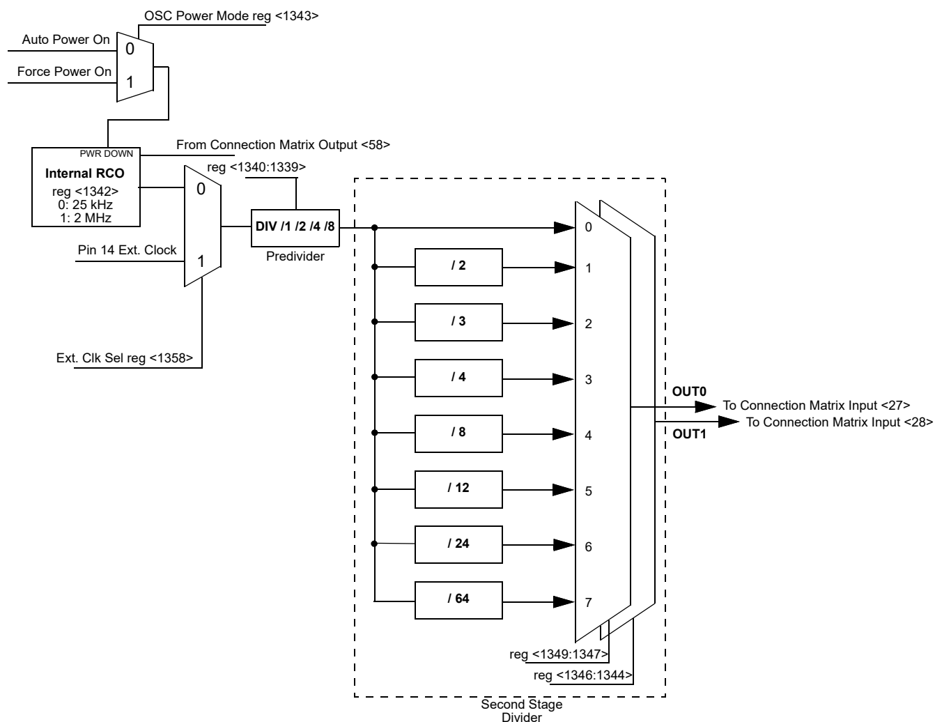
Figure 62. 25 kHz / 2 MHz RC OSC Block Diagram
