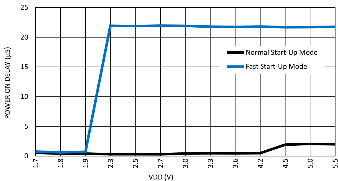
Figure 66. RC Oscillator Maximum Power On Delay vs. VDD at 85°C, OSC0 = 25 kHz
