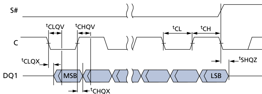
Figure 48: Output Timing for DTR
