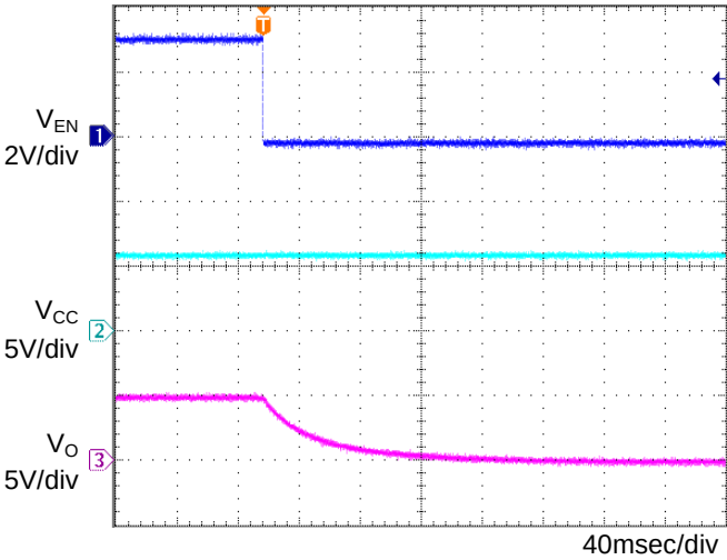
Figure 18. OFF sequence 2 C_o=1\mu\text{F} , T_a=-40^\circ\text{C}
