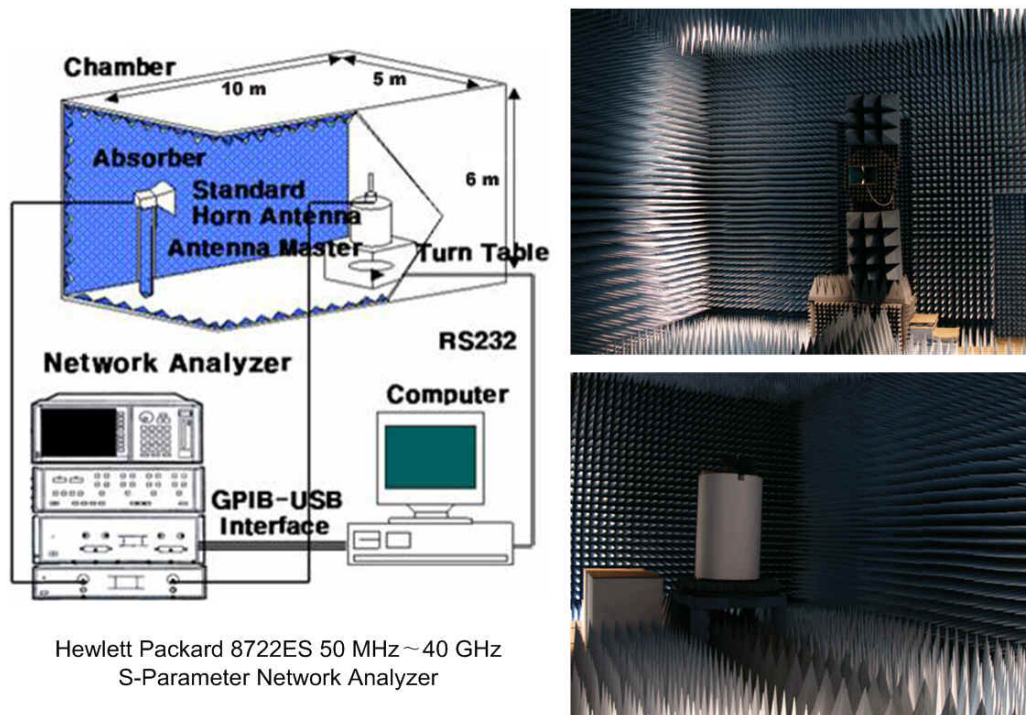
Fig 4. Measurement Configuration
