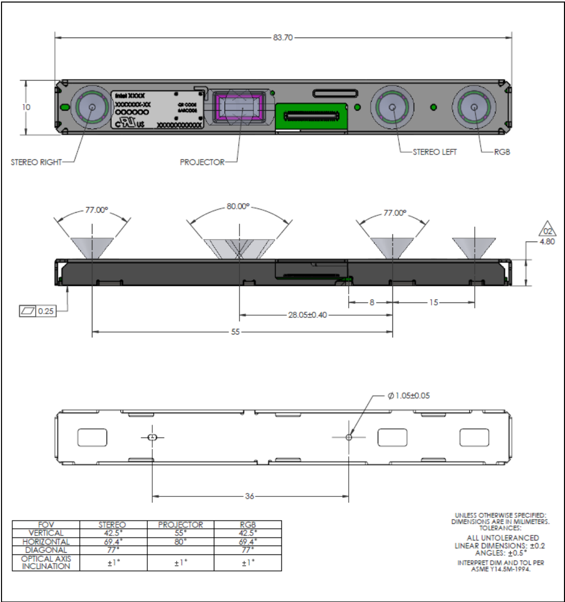
Figure 10-3. Intel ® RealSense ™ Depth Module D415
