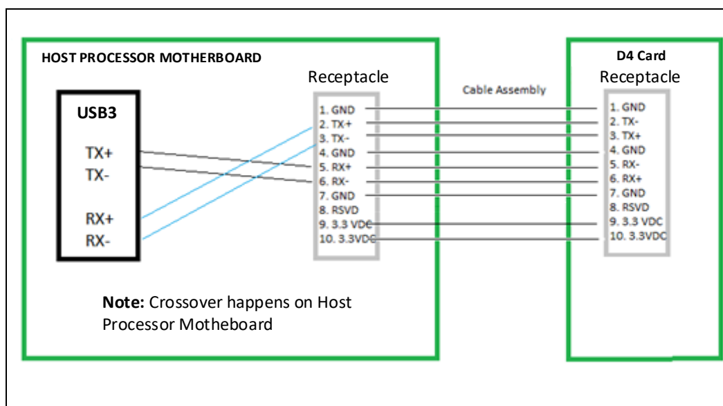
Figure 7-5. Host Motherboard USB 3.1 Gen 1 Routing
