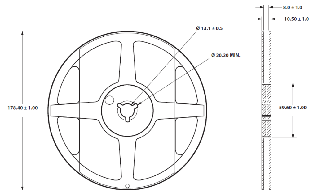
Figure 8: Reel Dimensions
