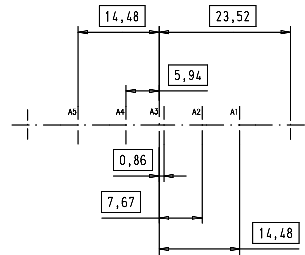
PCB layout hole, component side
