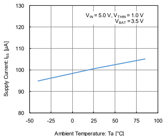
(14) Supply Current vs. Ambient Temperature
