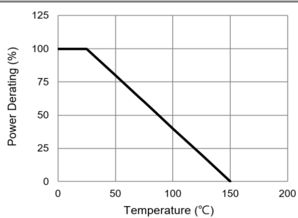
Fig.13 Gate-Total Power Dissipation
