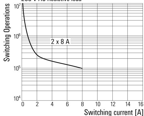
250 V AC Resistive load
