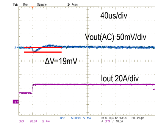
Step Load Transient Response (Vin=12V, Vout=1.8V, Cload=660uF, Iout=12A to 24A, 2.4A/us)
