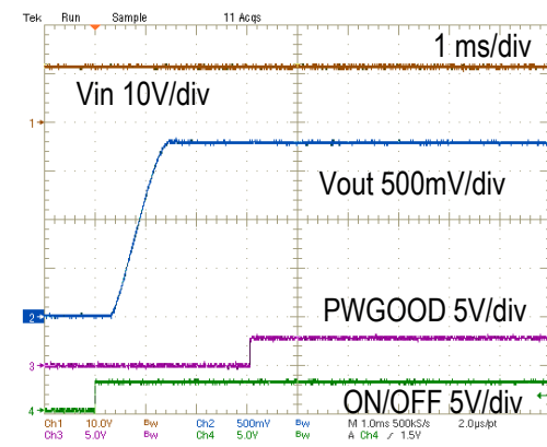
On/Off Enable Delay (Vin=12V, Vout=1.8V, Iout=24A, Cload=660uF)
