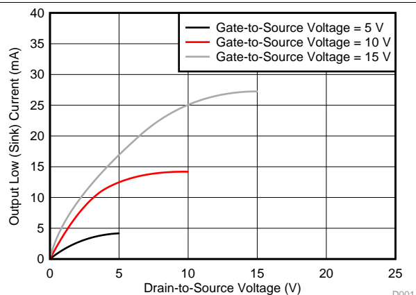
Figure 1. Typical Output Low (Sink) Current Characteristics
