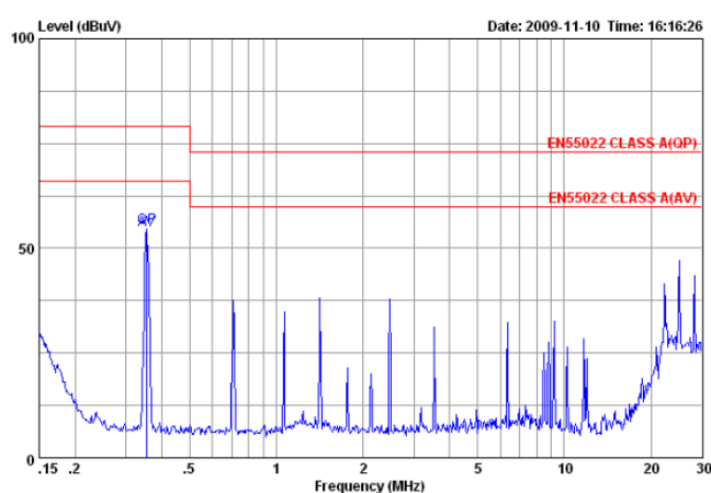
LISN connected to N Line
