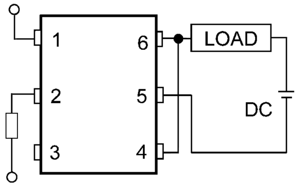
Fig. 14.3 C connection
