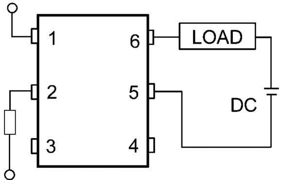
Fig. 14.2 B connection
