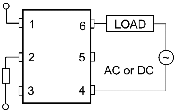
Fig. 14.1 A connection
