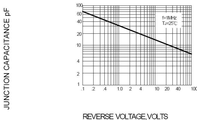
FIG.5-TYPICAL JUNCTION CAPACITANCE
