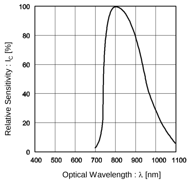
Fig.5 Spectral Sensitivity
