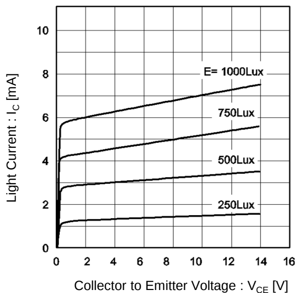
Fig.4 Output Characteristics
