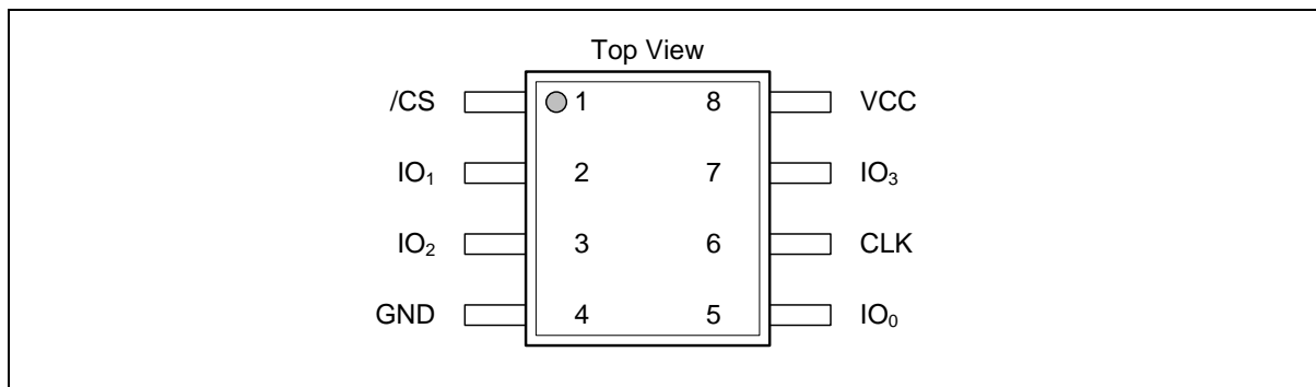
Figure 1a. W25R64JV Pin Assignments, 8-pin SOIC 208-mil (Package Code SS)
