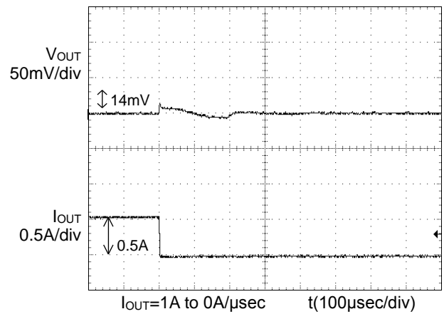
Figure 4. Transient Response (0.5 to 0A) C OUT =100μF, C FB =1000pF
