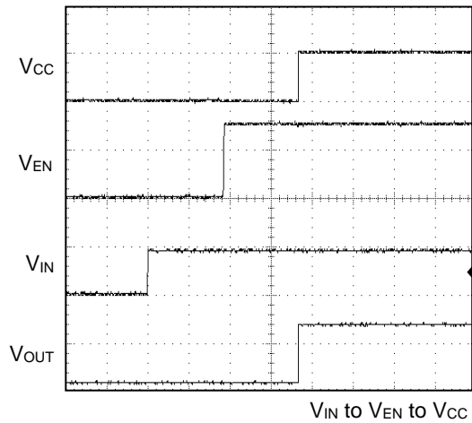
Figure 25. Input Sequence
