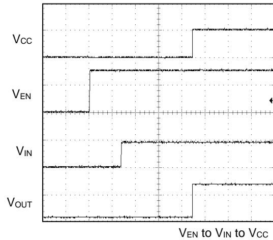
Figure 26. Input Sequence
