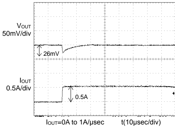
Figure 1. Transient Response (0A to 0.5A) C OUT =100μF, C FB =1000pF
