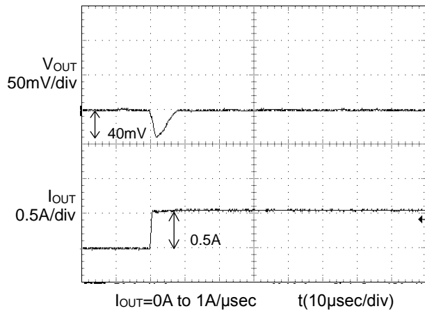
Figure 3. Transient Response (0A to 0.5A) C OUT =22μF, C FB =1000pF
