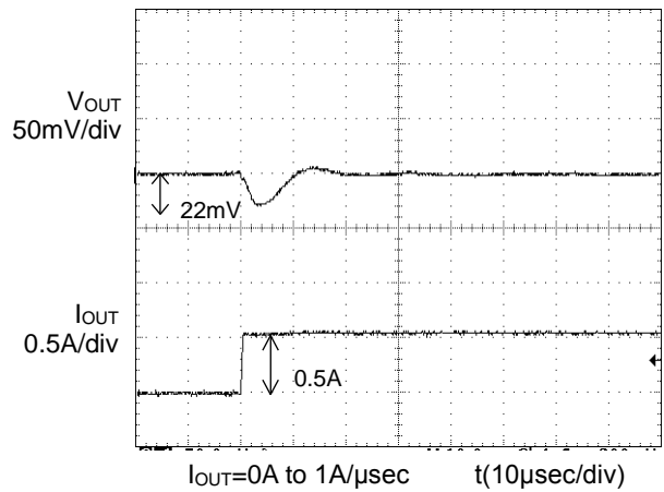
Figure 2. Transient Response (0A to 0.5A) C OUT =47μF, C FB =1000pF
