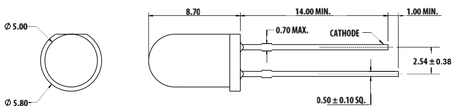
Figure 1: Package Drawing
