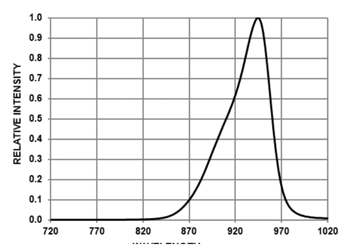
Figure 6: Spectral Distribution
