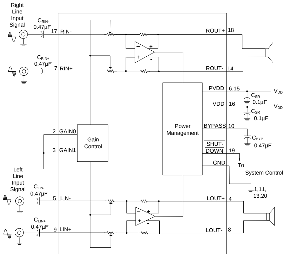
Fig.5 Differential inputs
