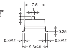
Raised actuator
