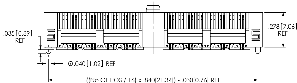
FIG 1 QFS-032-04.25-X-D-DP-A SHOWN
