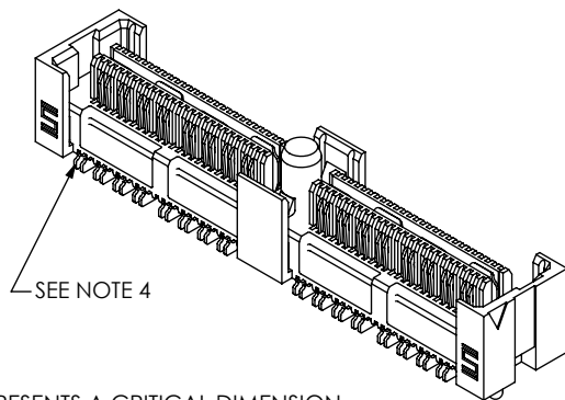
FIG 1 QFS-032-04.25-X-D-DP-A SHOWN
