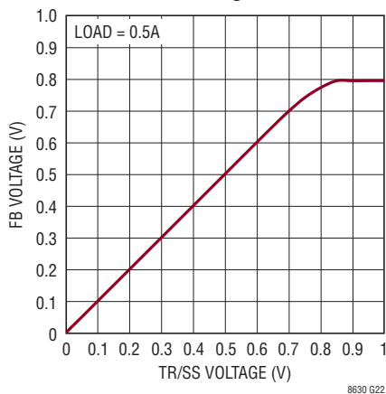
Soft-Start Tracking
