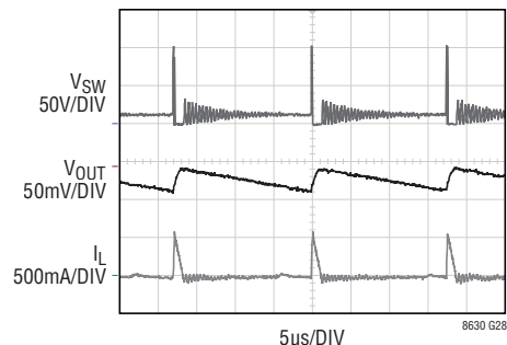
Burst Waveforms
