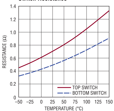
Switch Resistance
