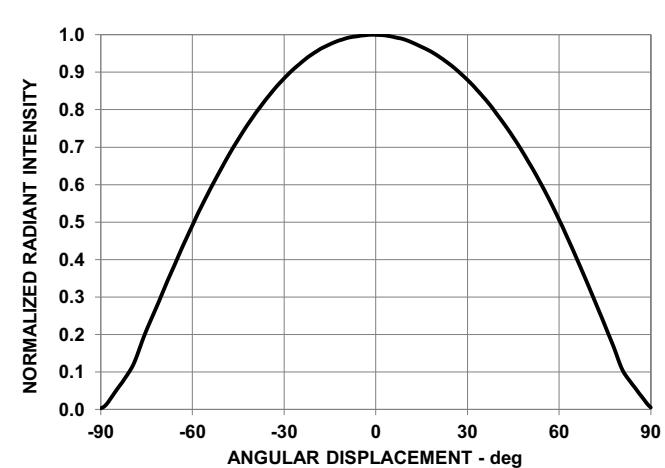
Figure 5: Radiation Pattern
