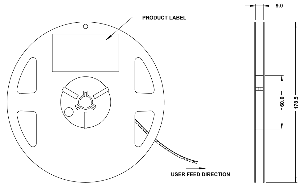
Figure 11: Reel Dimensions
