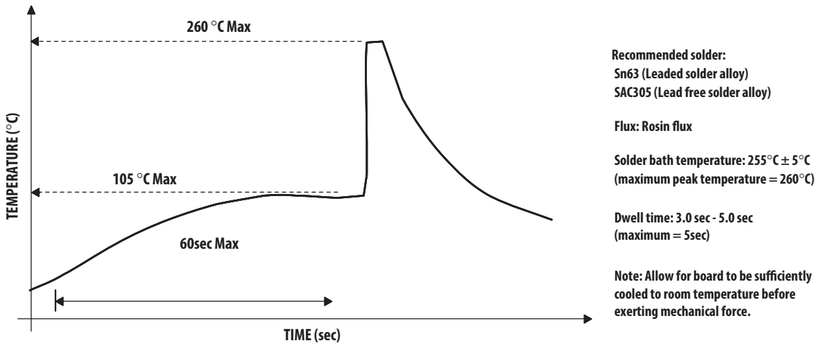
Figure 12: Example of Wave Soldering Temperature Profile for TH LED
