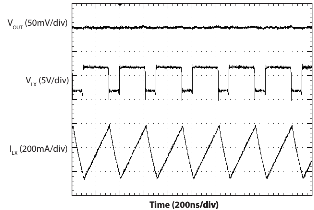
Heavy Load Switching — V_{OUT} = 3.3V
