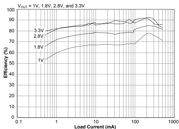
Efficiency vs. I_{OUT} ( T_A = -40^\circ C )
