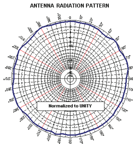
Representative Azimuth Field Pattern
