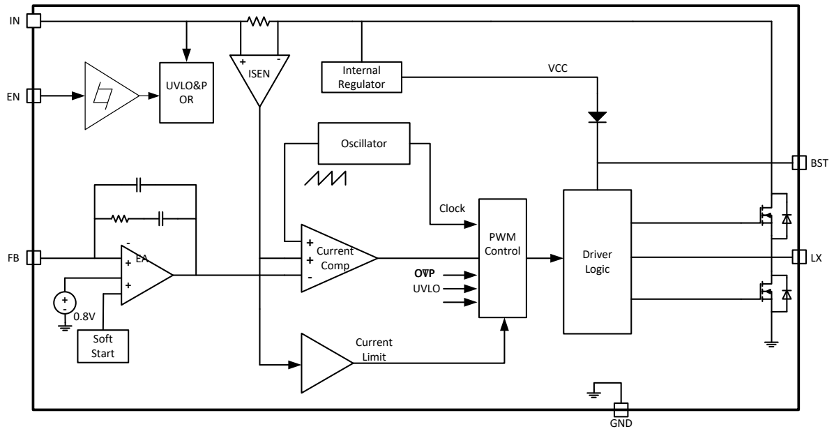
Figure 2. MSMP1470BGJ-Z Block Diagram
