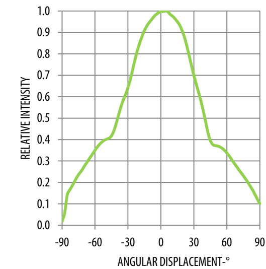
Figure 5: Radiation Pattern
