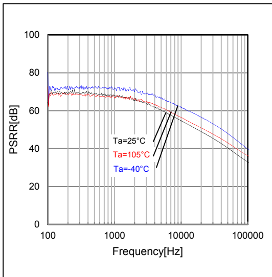
Figure 24. PSRR (Input Voltage Ripple = 1Vrms, I_o = 50\text{mA} )
