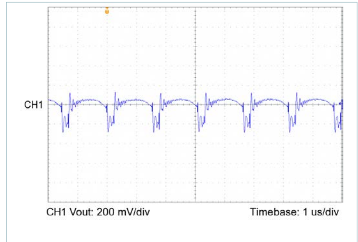
Figure 18 — Output voltage ripple, V_{IN} = 100\text{V} , V_{OUT} = 5.0\text{V} , C_{OUT\_EXT} = 1000\mu\text{F} , R_{LOAD} = 0.208\Omega
