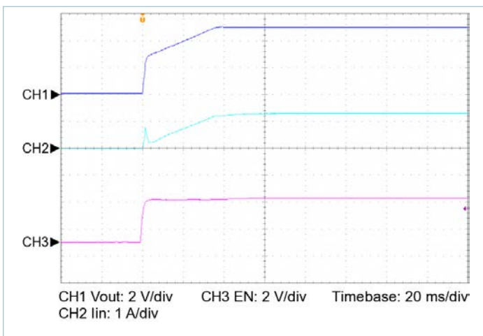
Figure 19 — Start up from EN, V_{IN} = 100\text{V} , C_{OUT\_EXT} = 20000\mu\text{F} , R_{LOAD} = 0.208\Omega
