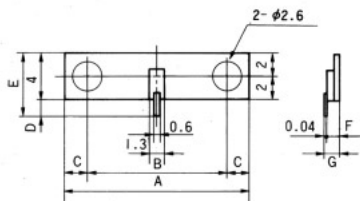
PCB Mounting Pattern
