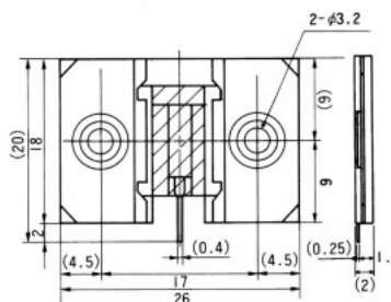
PCB Mounting Pattern
