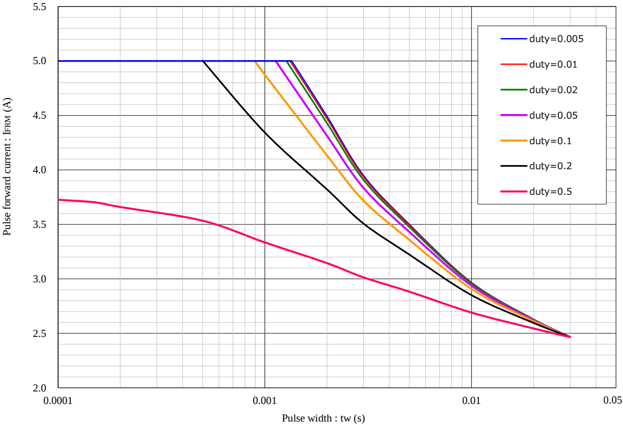
Maximum ratings of pulse forward current Condition : T_s = 85^\circ\text{C}
