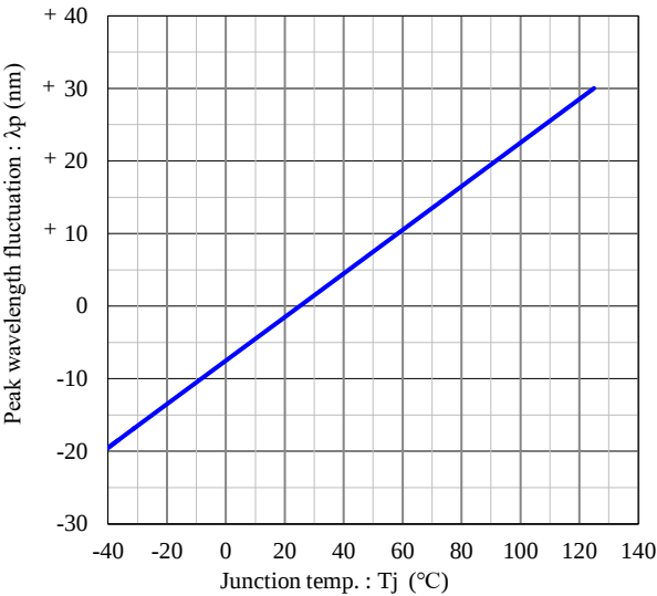
Junction temp. vs. Peak wavelength fluctuation Conditions : If = 1A
