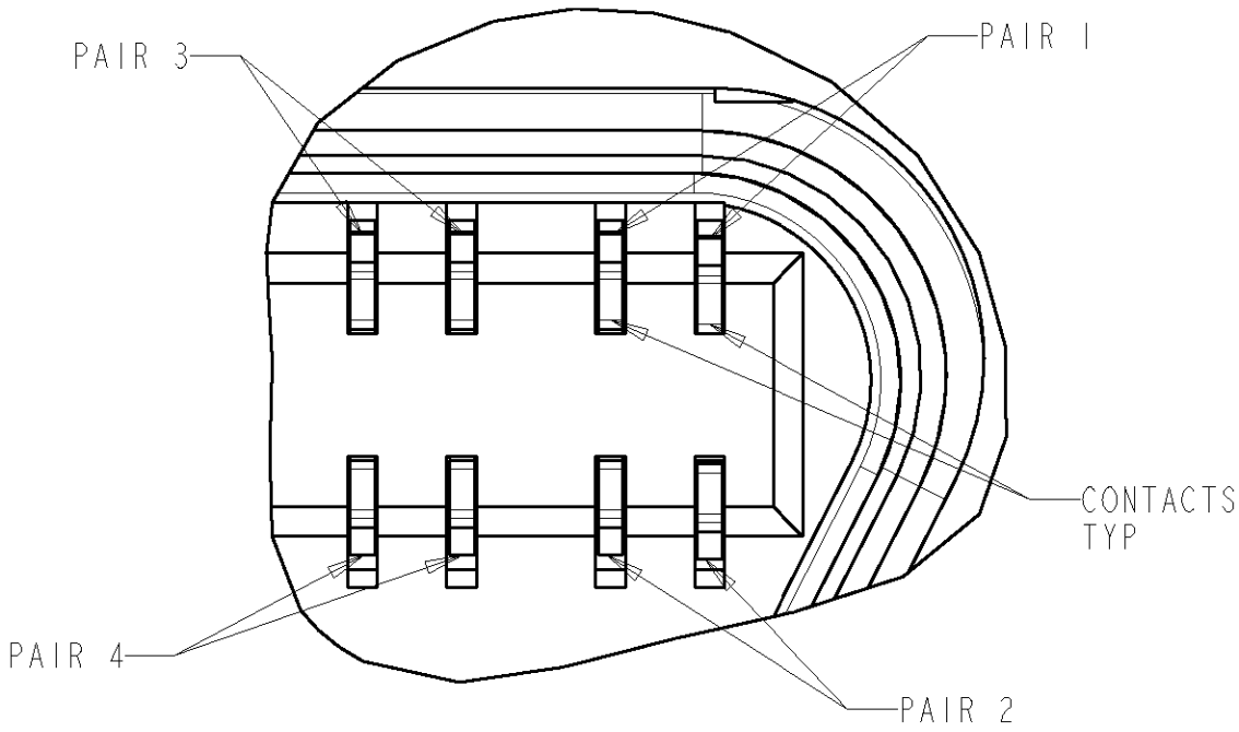
DETAIL M SCALE 12:1
