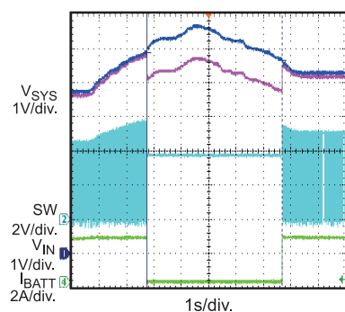
Input Over Voltage Protection, Charge Mode
