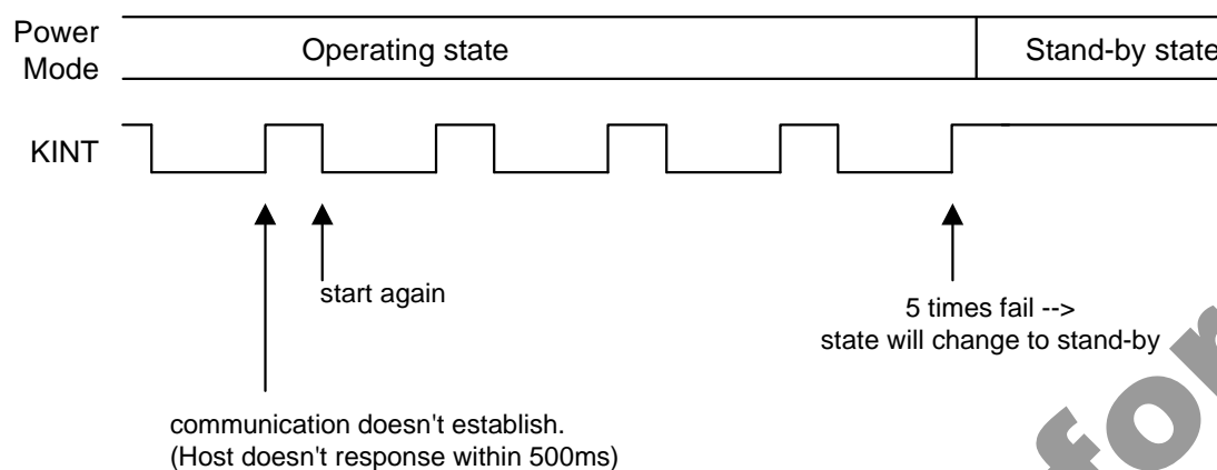
Fig.6 3wire timeout
