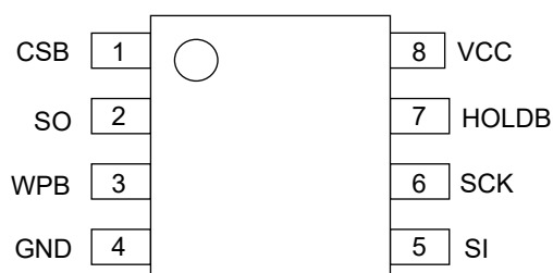
Figure 3-(a). Pin Configuration (SOP8, SOP-J8, TSSOP-B8, MSOP8)
