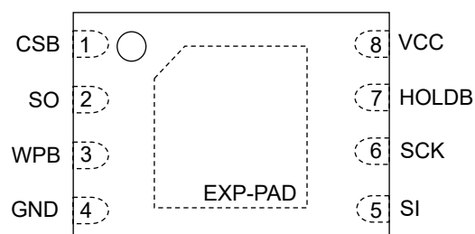
Figure 3-(b). Pin Configuration (VSON008X2030)
