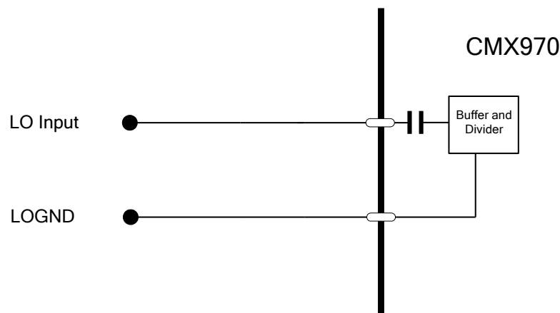
Figure 4 LO Input Configuration
