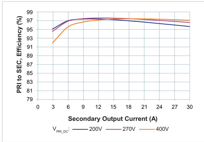
Figure 10 — Efficiency at T_{CASE} = 100^{\circ}\text{C}
