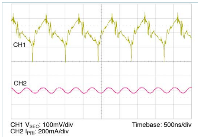
Figure 14 — Full-load secondary voltage and primary current ripple, 10\mu\text{F } C_{PRI\_IN\_EXT} ; no external C_{SEC\_OUT\_EXT} . Board-mounted module, scope setting: 20MHz analog BW
