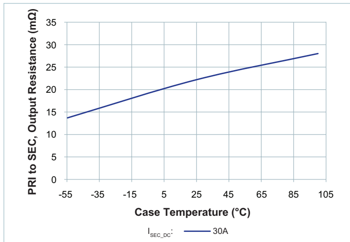
Figure 12 — R_{SEC} vs. temperature; nominal V_{PRI\_DC} I_{SEC\_DC} = 30\text{A} at T_{CASE} = 100^{\circ}\text{C}
