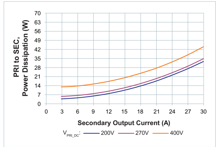
Figure 11 — Power dissipation at T_{CASE} = 100^{\circ}\text{C}
