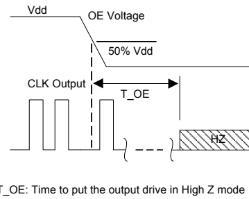
Figure 7. OE Disable Timing (OE Mode Only)
